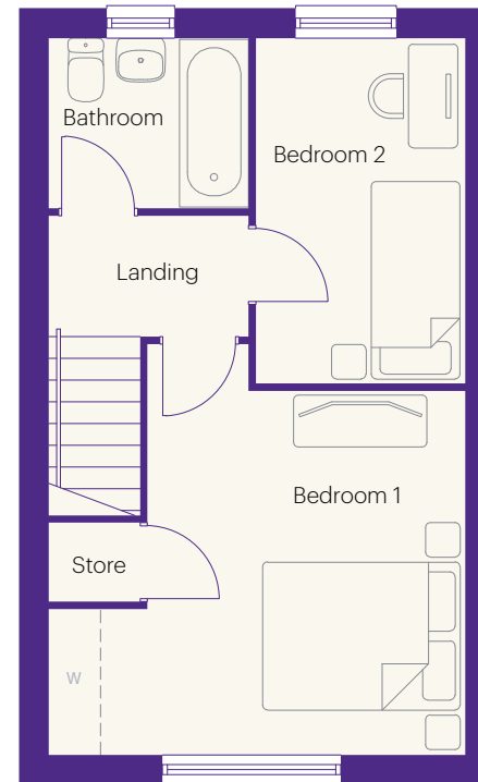
First floor dimensions
