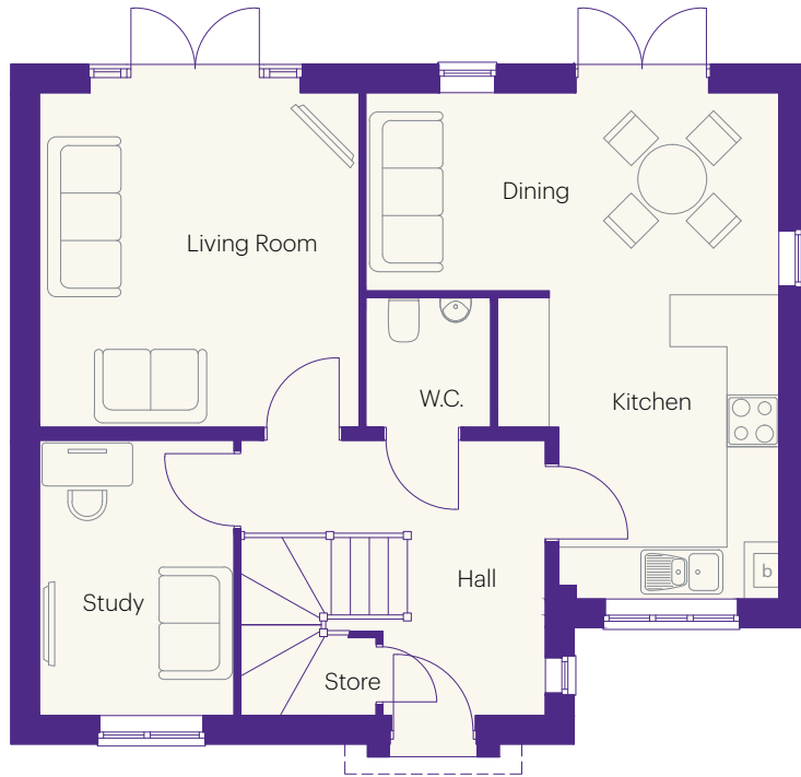
Ground floor dimensions
